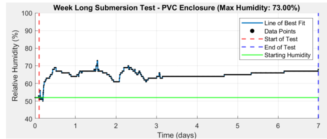
(b) Humidity tracking over the PVC enclosure over a 7 day field test
