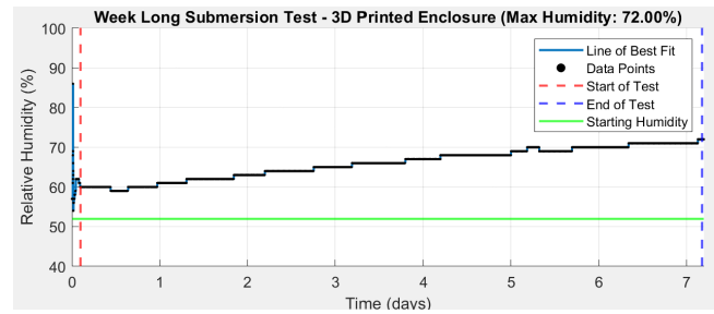
(a) Humidity tracking over the 3D printed enclosure after a 7 day field test
