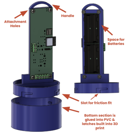
Figure 5: Node insert
