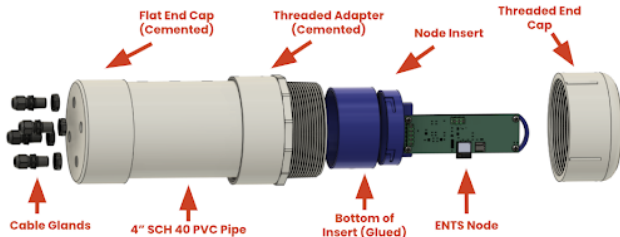
Figure 7: Exploded view of PVC enclosure
