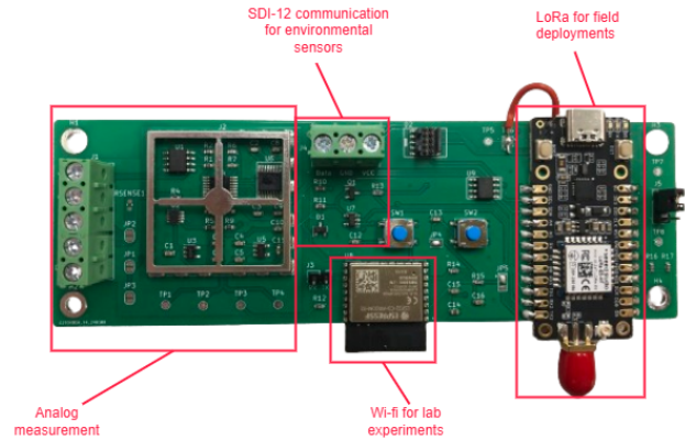
Figure 2: An ENTS node. A typical deployment might involve dozens of ENTS nodes collecting SMFC data in laboratory settings over WiFi before being transitioned to outdoor deployments, where data transmission occurs via LoRa.
