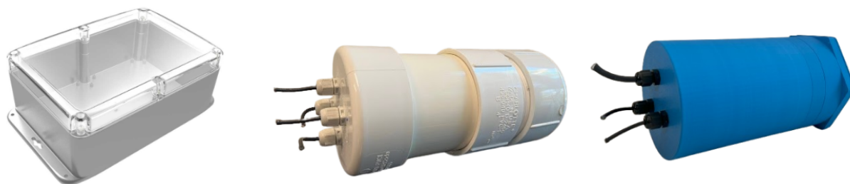
Figure 1: Three different environmental enclosure options for sensing platforms. From left to right: an industry standard, commercial-off-the-shelf IP68 box, our custom PVC enclosure, and our custom 3D printed enclosure.
