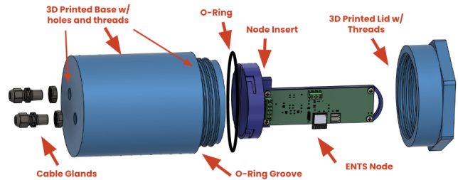
Figure 6: Exploded view of 3D printed enclosure
