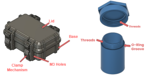
Figure 3: Two 3D printed enclosure designs: clamping box, hex screw-sealed tube
